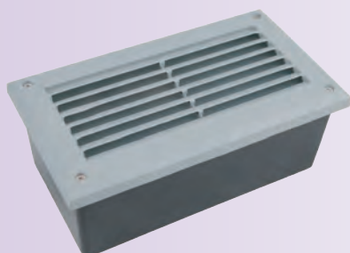
Ref-BRL-BH-5000-001 Stair Light LED Wattage :5W Dimensions :225mm CCT: 6000K
