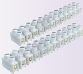
Terminal Connector (Plastic) Size : 6 / 8 / 10 mm
