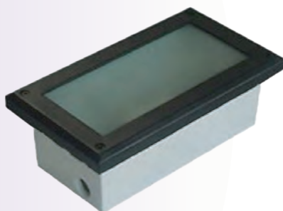
Ref-BRL-BH-5003-001 Stair Light LED Wattage :5W Dimensions :228mm CCT: 6000K
